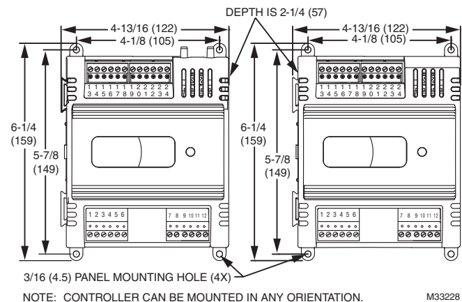
Fig. 1. Panel mounting—controller dimensions in inches (mm) for PUB1012S, PUB4024S, and PVB4024NS only (PUB4024S and PVB4024NS shown).
