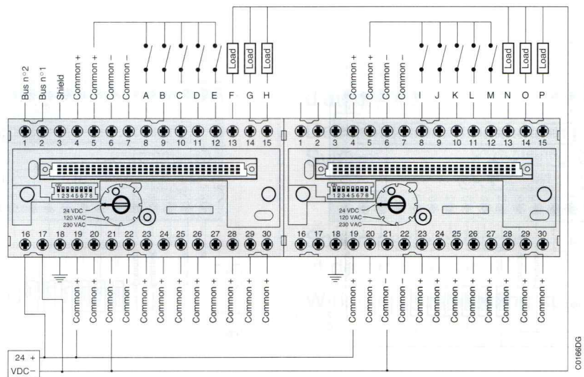
Type / Unit : 24 VDC ICSC 08 L1 Binary input / output module
