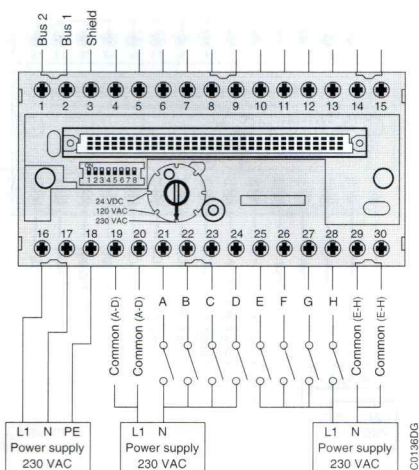
Type / Unit : 120 VAC / 230 VAC ICSC 08 L1 Binary input / output module
